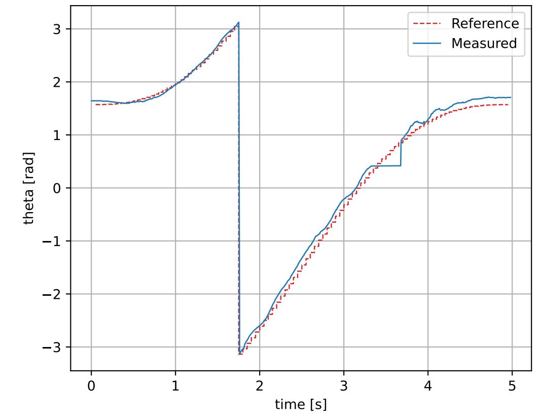
theta State
